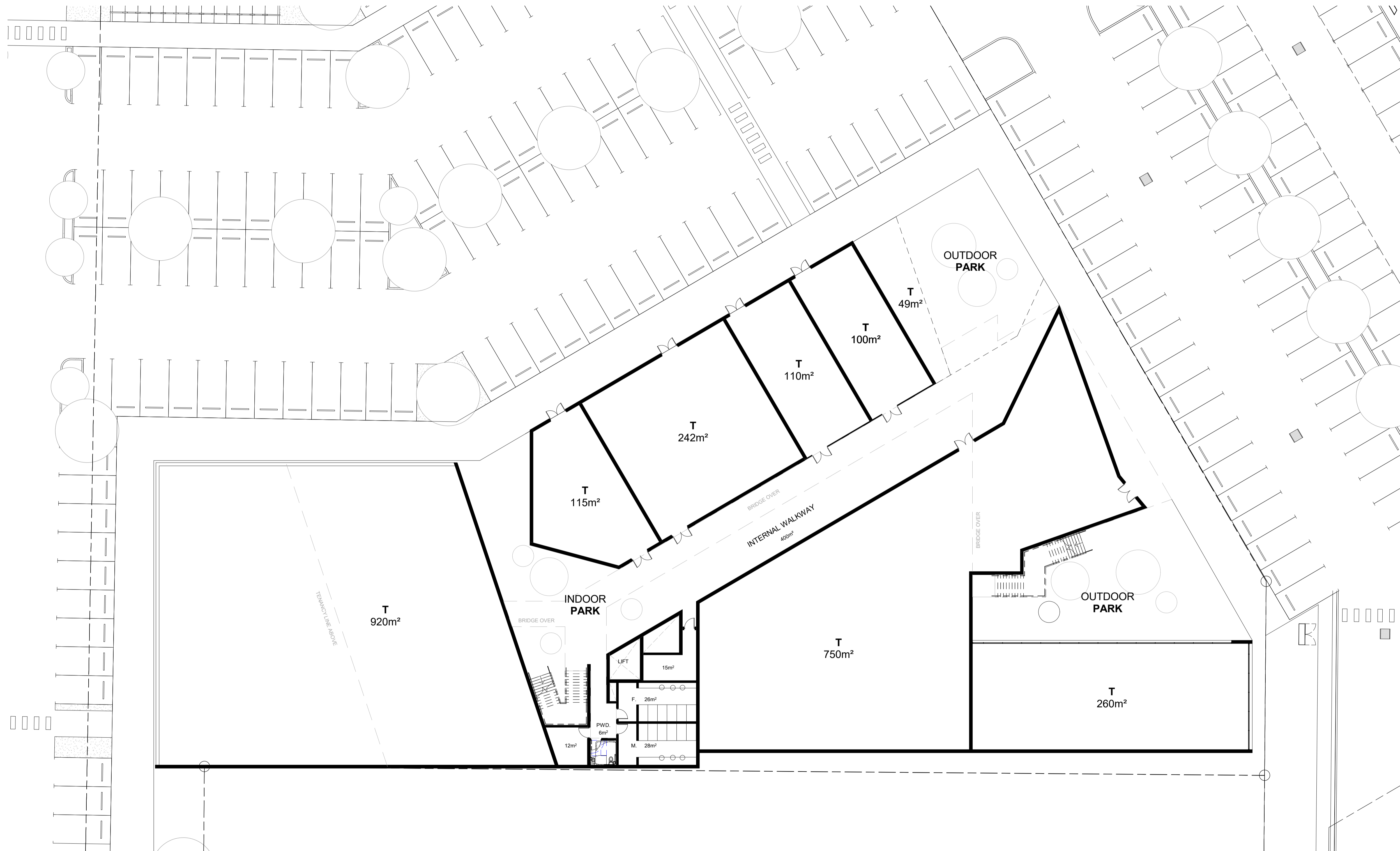
GROUND FLOOR PLAN 1:200
